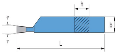
Technical drawing of a parting off tool.
