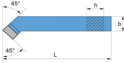
BENT TURNING TOOL
