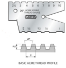
BASIC ACME THREAD PROFILE
